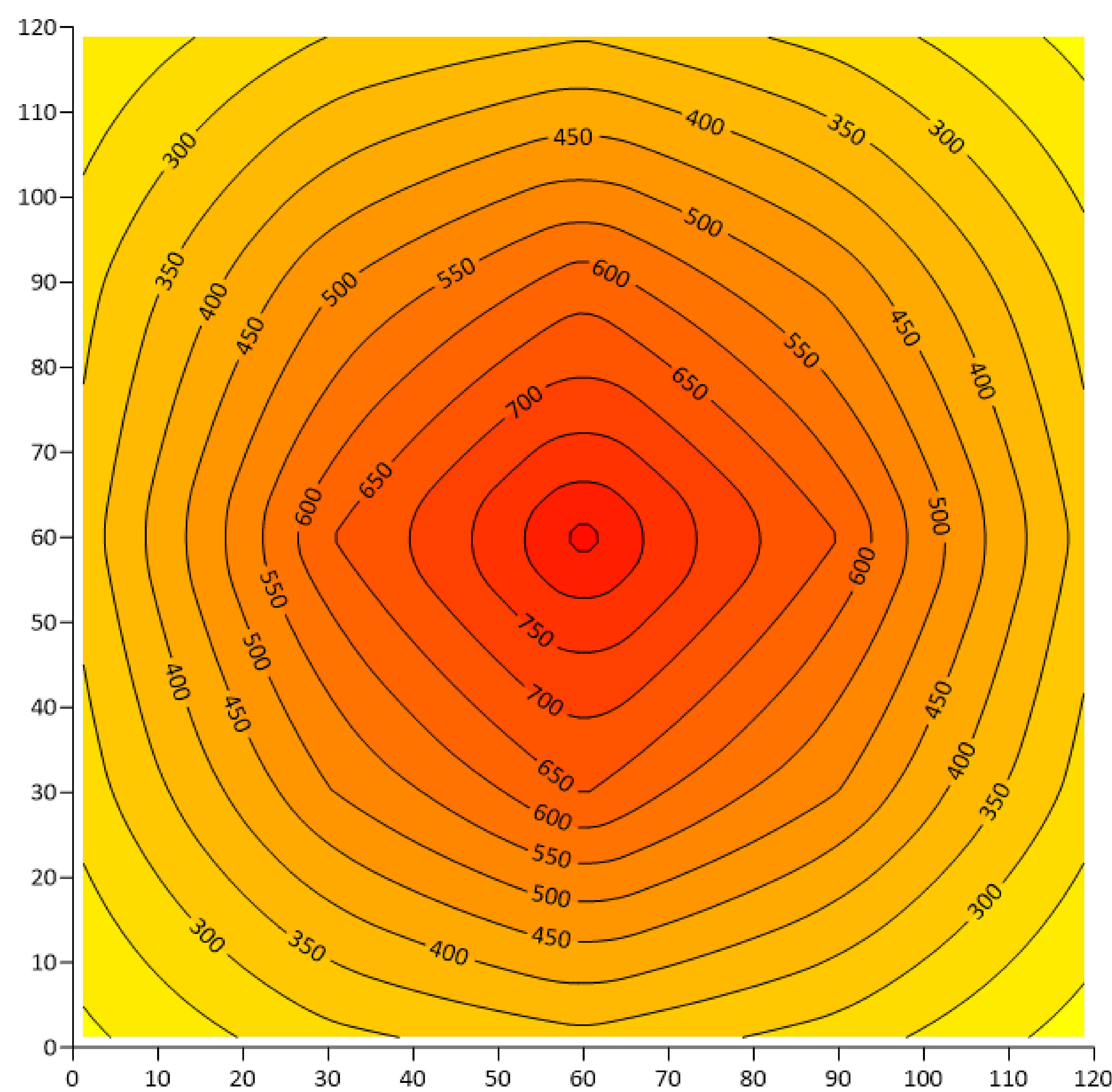
Pro-240W DEEP RED a 0,5m
